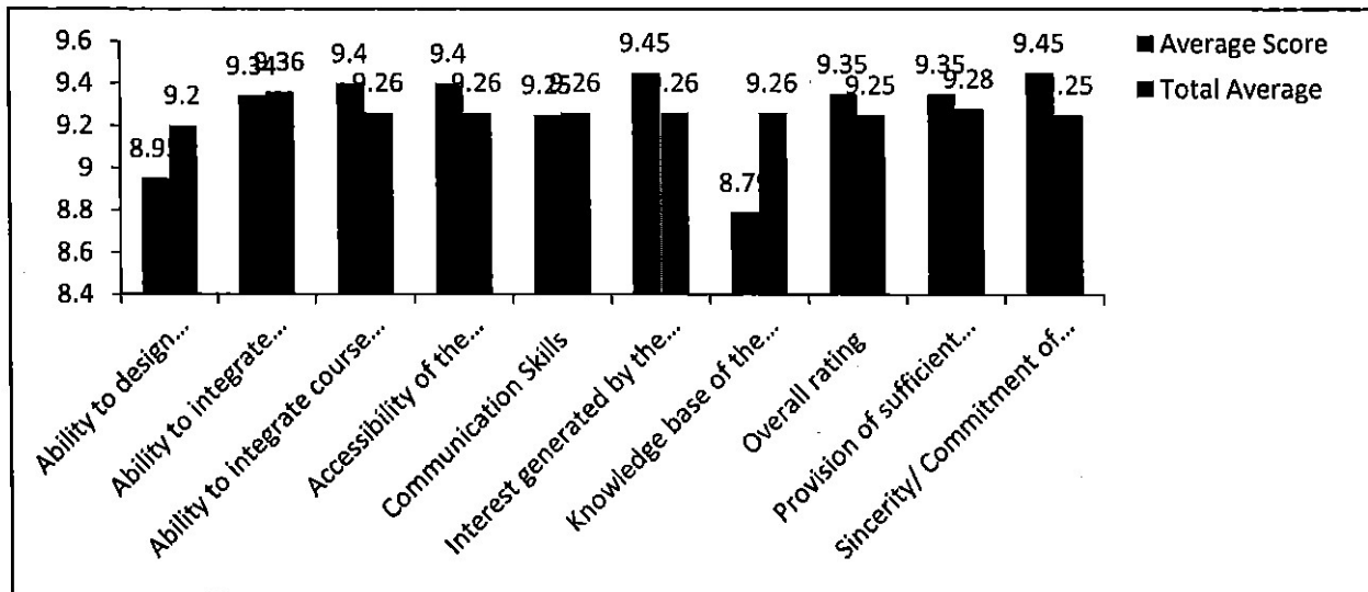
Figure 6: Bar Spline Diagram-comparison based on average score
