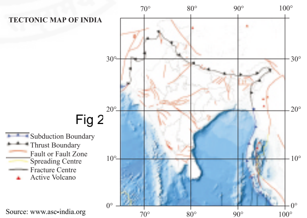
Fig 2.1.5 Fault lines in India
