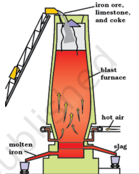
Fig. 5.6: From iron ore to steel in a blast furnace
